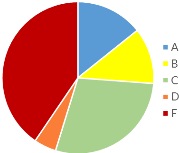
Grade Distribution Unhealthy Particle Days SOTA 2018
