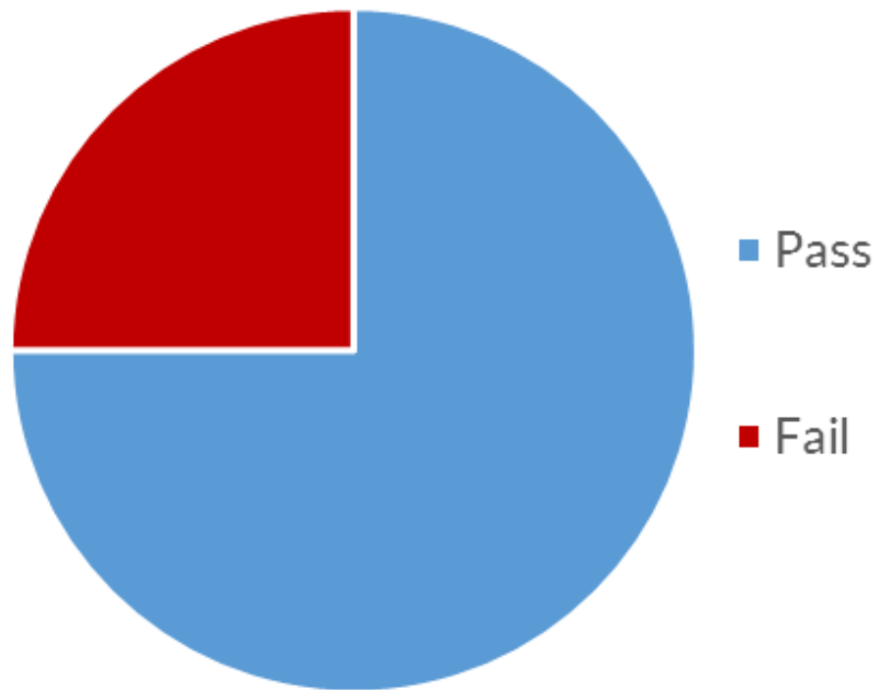
Grade Distribution Annual Particle Pollution SOTA 2018
